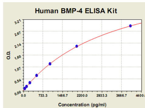
Figure 1: BMP-4 Standard Curve. Using the Human BMP-4 ELISA Kit, O.D. data was graphed against BMP-4 protein concentration. The TMB reaction was incubated at 37°C for 18 min.
