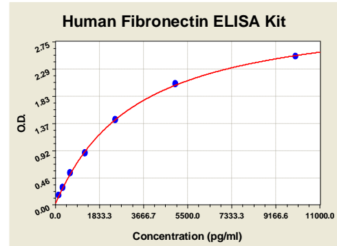
Figure 1: Fibronectin Standard Curve. Using the Human Fibronectin ELISA Kit, O.D. data was graphed against Fibronectin protein concentration. The TMB reaction was incubated at 37°C for 17 min.
