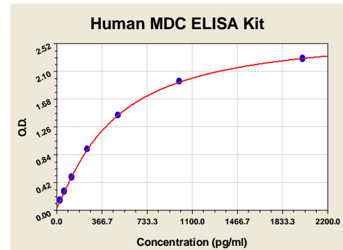
Figure 1: MDC Standard Curve. Using the Human MDC ELISA Kit, O.D. data was graphed against MDC protein concentration. The TMB reaction was incubated at 37° C for 13 min.
